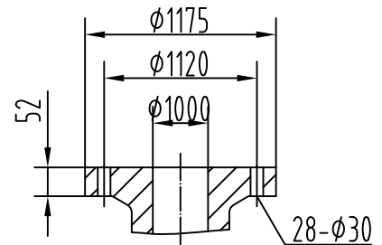
Outlet Flange (0.6Mpa)
