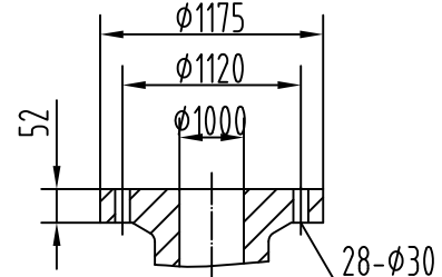
Outlet Flange (0.6Mpa)
